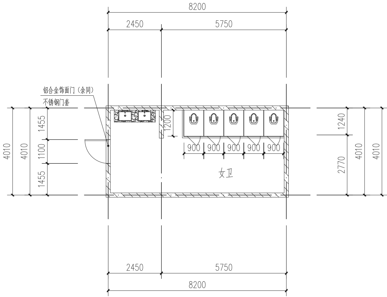
仰仪南楼（女卫）卫生间 1:100
