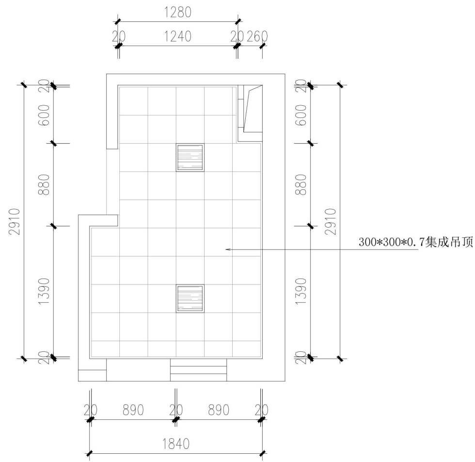
宿舍卫生间顶面图
