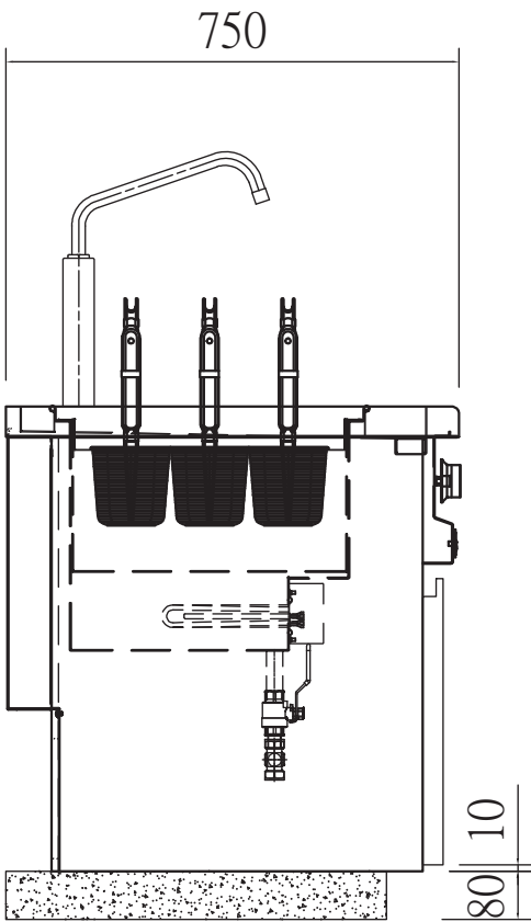
SIDE VIEW
