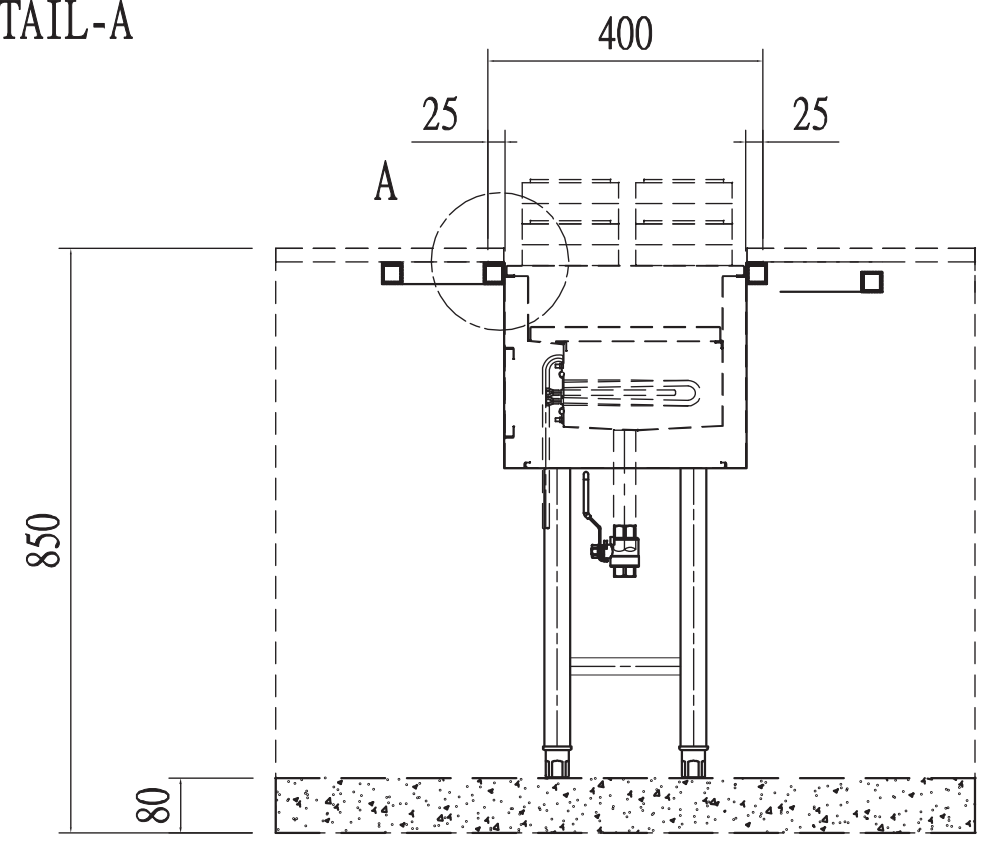
SIDE VIEW
