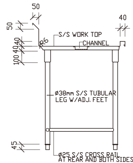
SECTION
