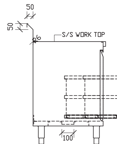
SECTION
