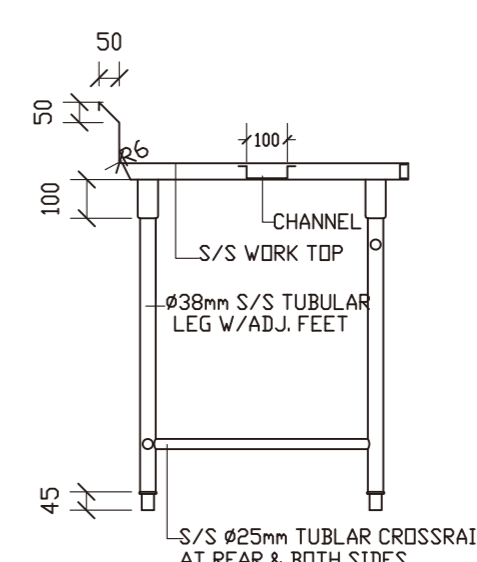
SECTION
