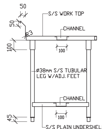
SECTION
