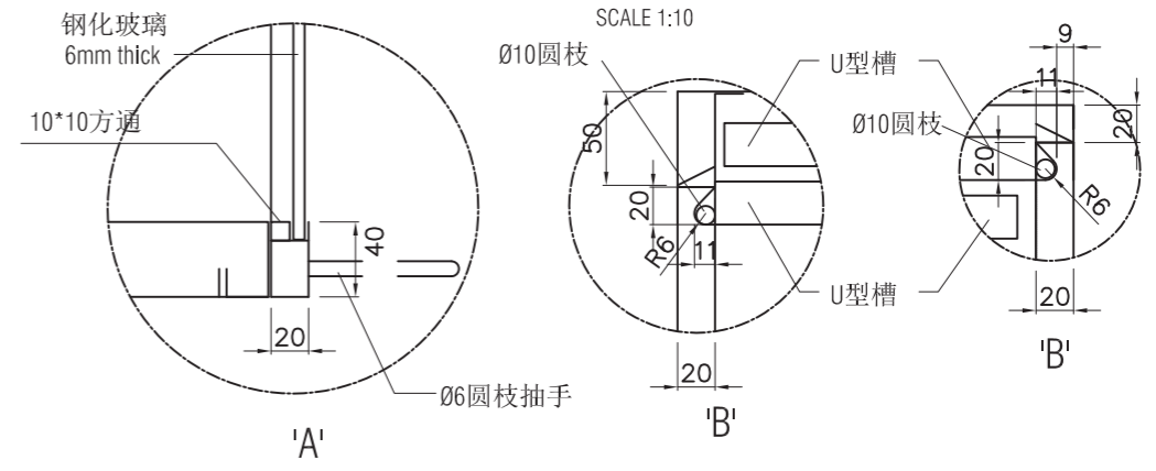
SECTION A
