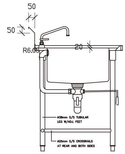
SECTION
