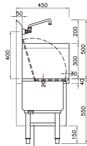
SECTION A
