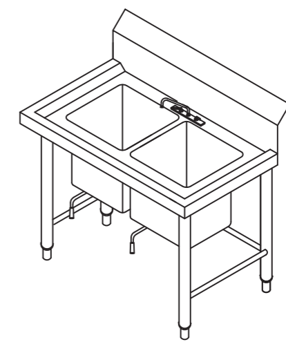
ISOMETRIC VIEW
