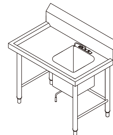
ISOMETRIC VIEW
