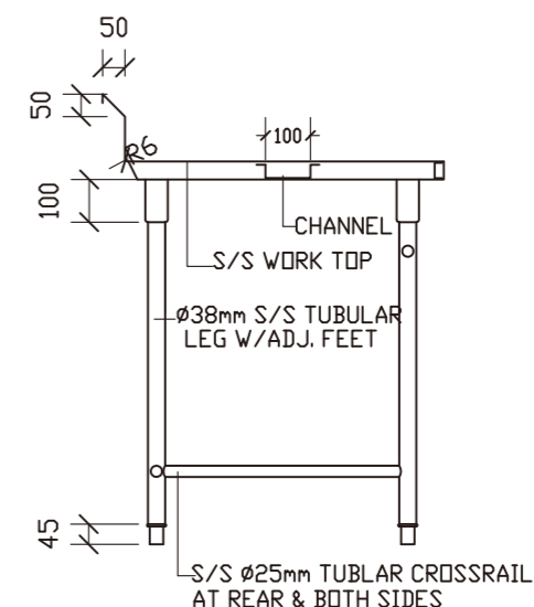
SECTION
