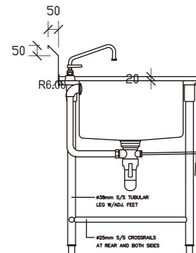
SECTION
