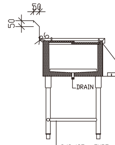
SECTION
